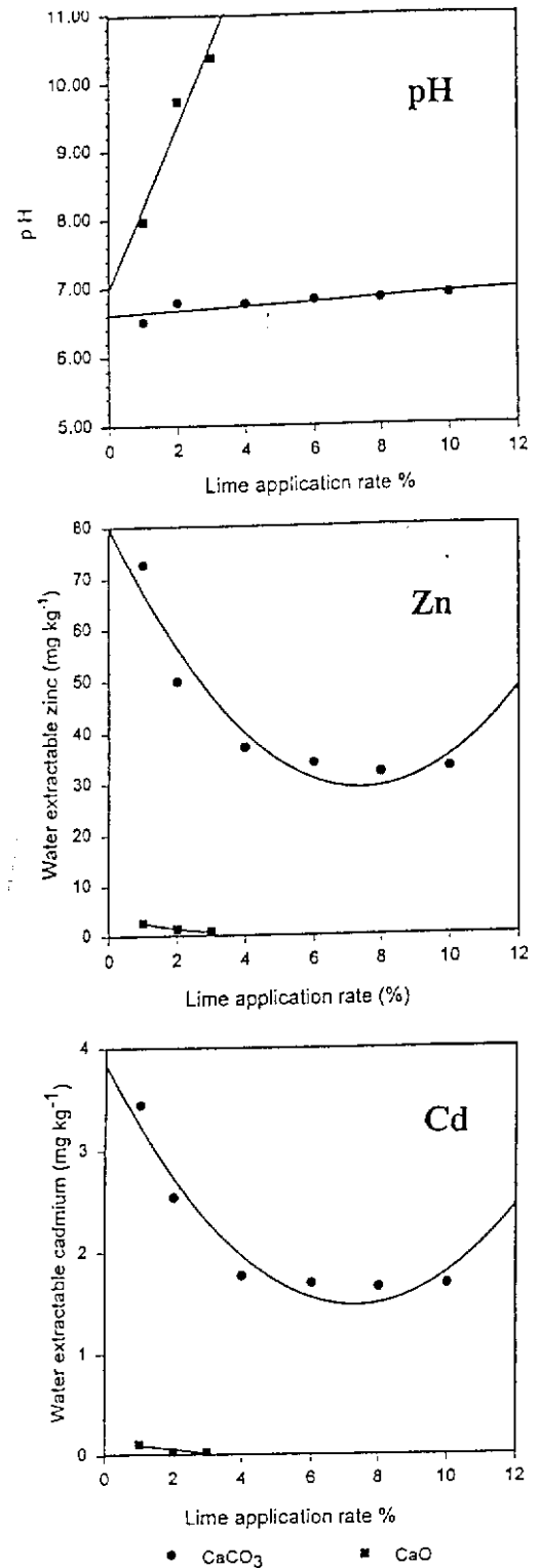
Figure 3. Influence of lime rate and type on pH and water soluble metal levels in Welz waste. These relationships point out the importance of driving the pH to levels > 7.0 to limit Zn and Cd solubility, even though the original pH was 6.6. The data also point out the relative inability of \text{CaCO}_3 alone to affect pH in this metalliferous system.
