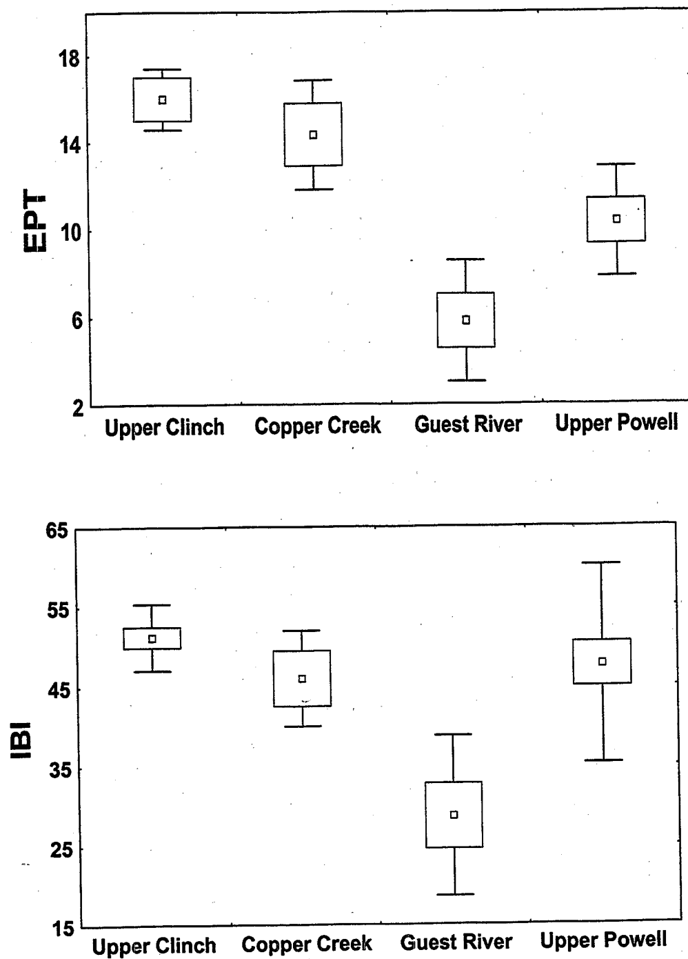
Figure 5-12. Macroinvertebrate (EPT) and fish (IBI) community integrity scores by subwatershed in the Clinch and Powell watershed based on TVA's CPRATS dataset. Boxes represent standard errors of the mean and whisker bars represent standard deviations of the mean.
