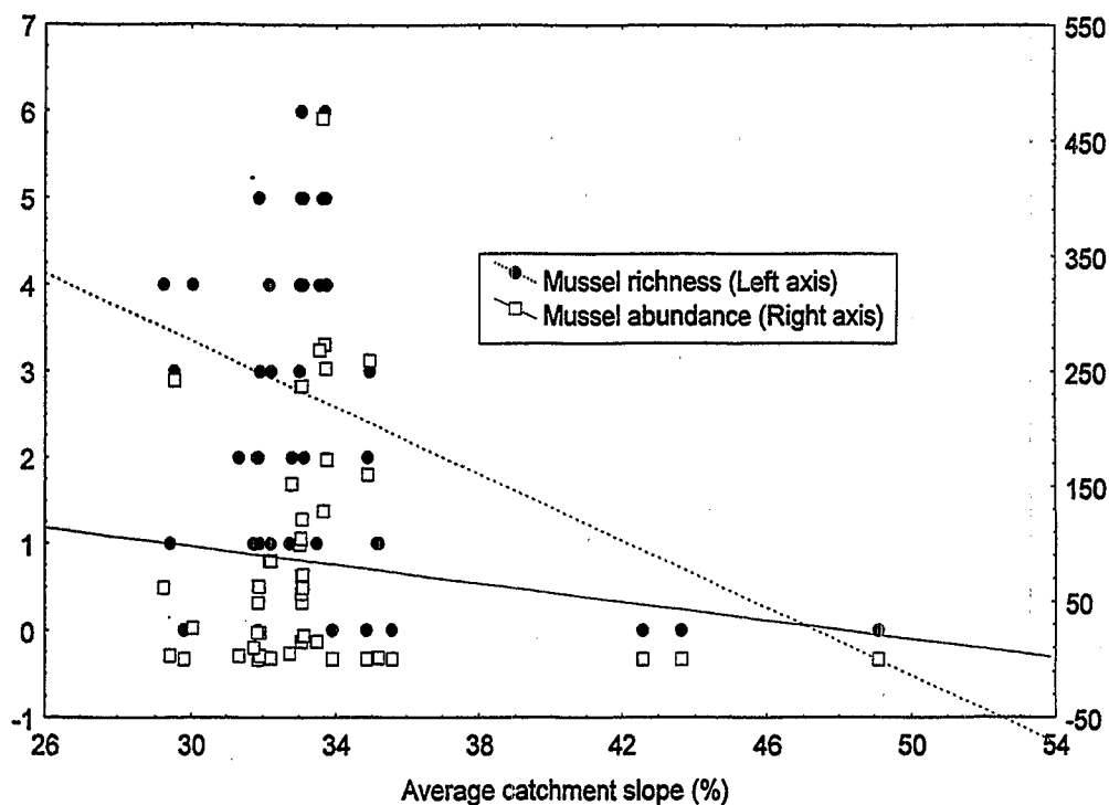
Figure C-11. Relation of mussel richness (left Y-axis) and abundance (right Y-axis) to average catchment slope (%) for low-order streams (3 rd or 4 th order).
