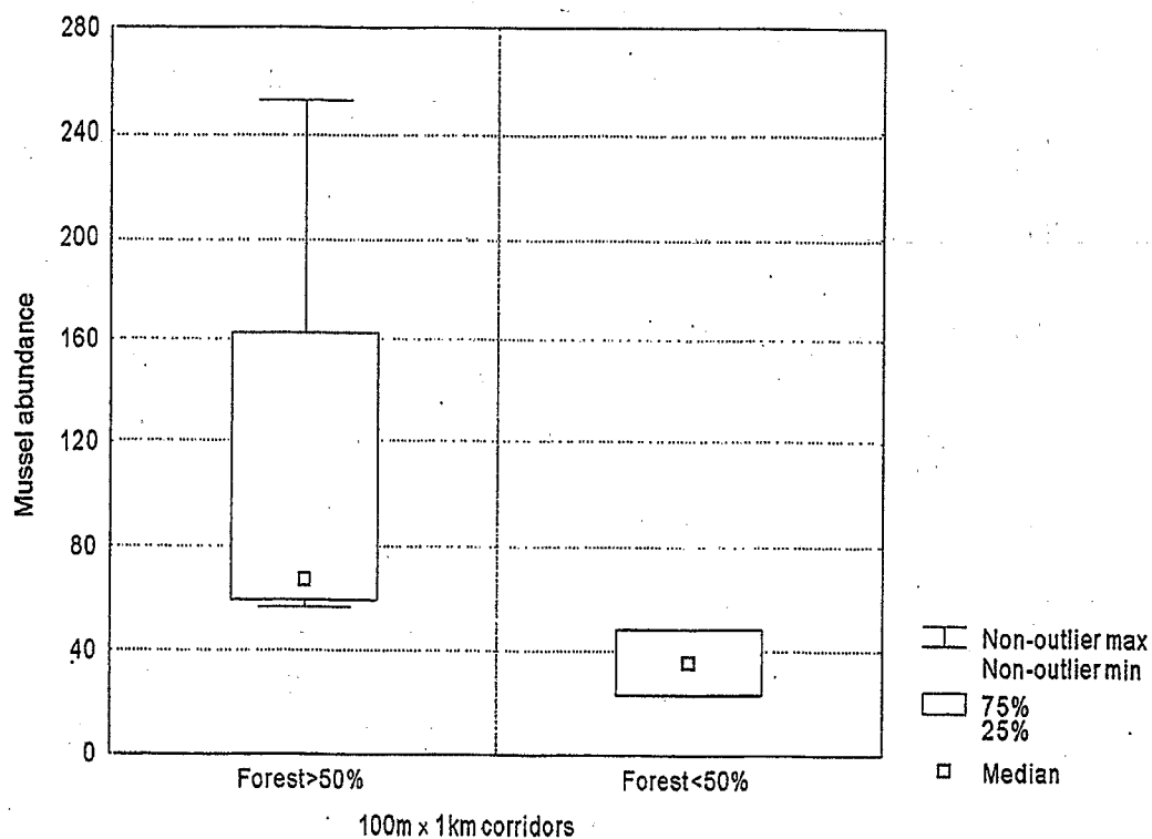
Figure C-5. Abundance of mussels in relation to forested land within 100-m-wide, 1-km-long riparian corridors of high-order streams (>4 th order).
