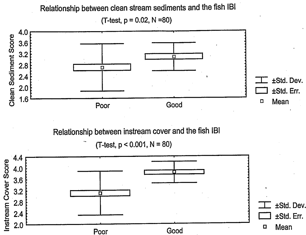
Figure 5-10. Relationship between stream embeddedness or cover and the fish IBI, categorized as either poor (impaired) or good (unimpaired), based on TVA's criteria.
