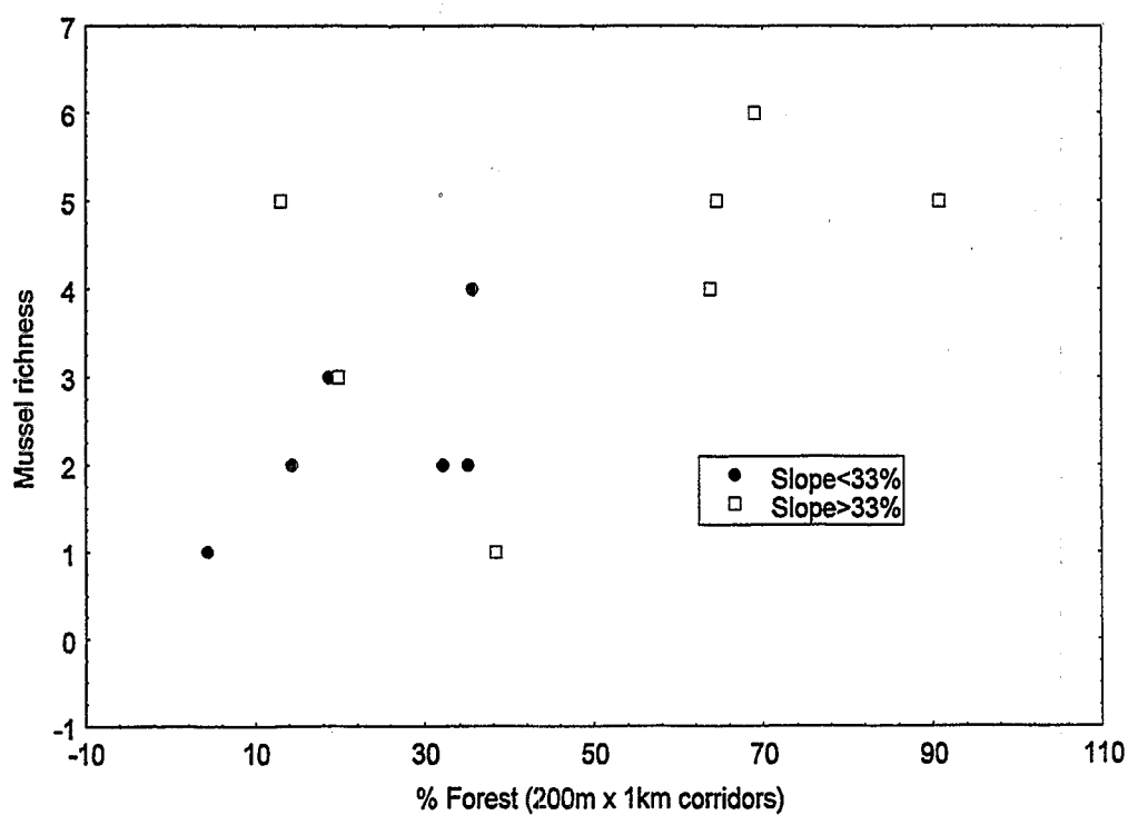
Figure C-2. Mussel richness versus the percentage of forested land within 200-m- wide, 1-km-long riparian corridors; streams are separated according to an average catchment slope threshold of 33%.
