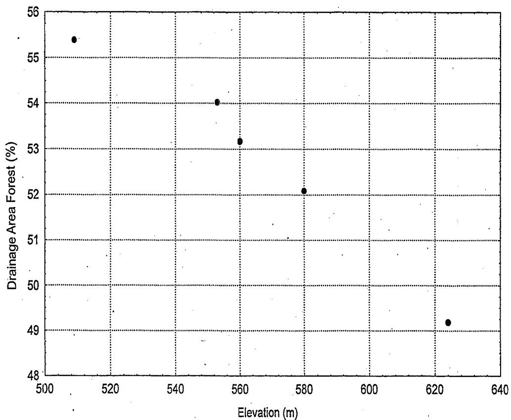
Figure C-10. Drainage area forested land (%) versus site elevation for high-order streams (>4 th order).
