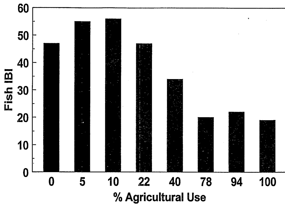
Figure 4-4. Fish community integrity as a function of agricultural land in the riparian corridor (riparian corridor defined as 100 m to either side of the stream and 1,500 m upstream).
