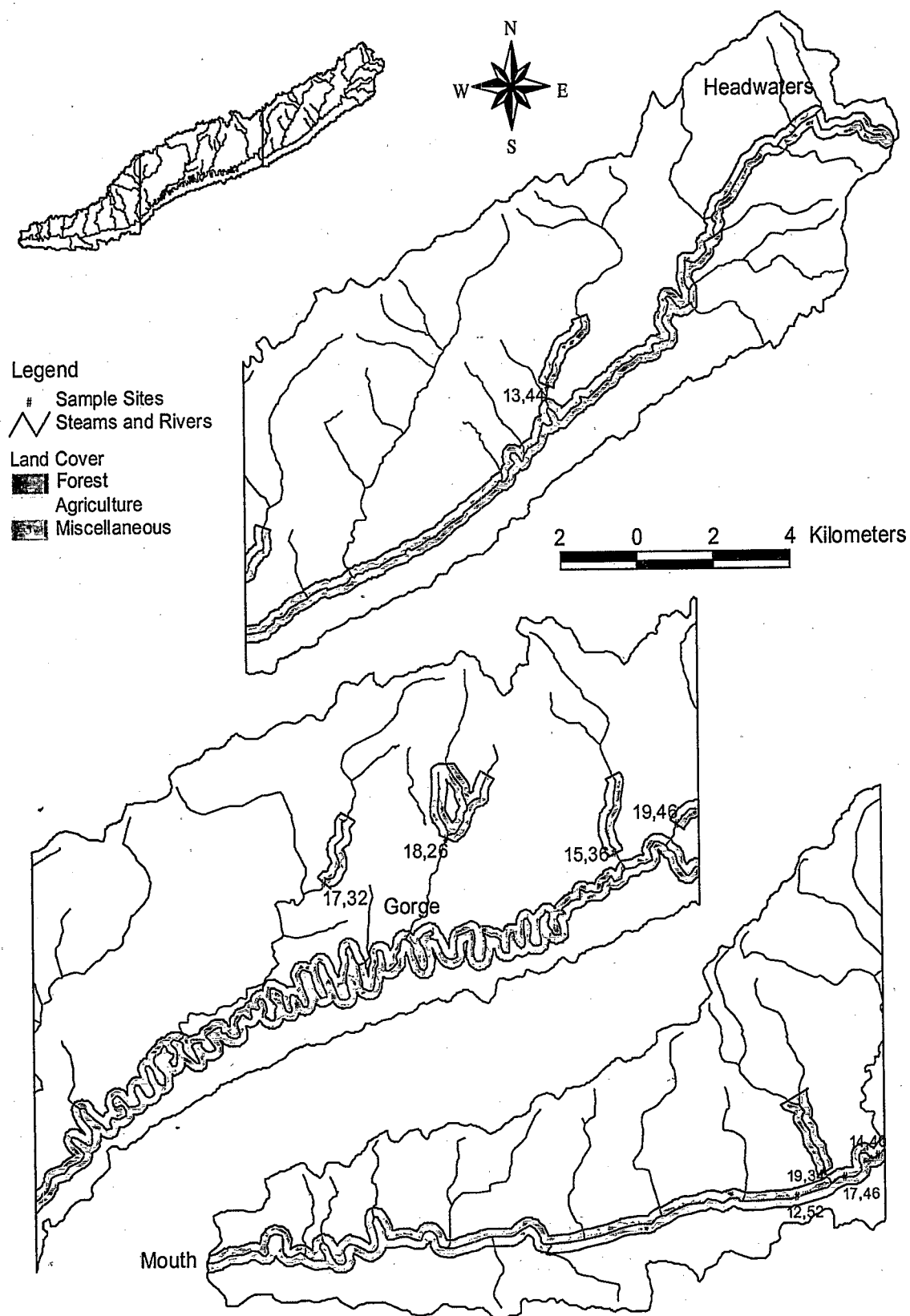
Figure 4-6. Forest and agricultural uses in the riparian corridor (200 m wide) of Copper Creek. Numbers represent macroinvertebrate EPT score and fish IBI values in TVA's CPRATS database, 1995–1996.
