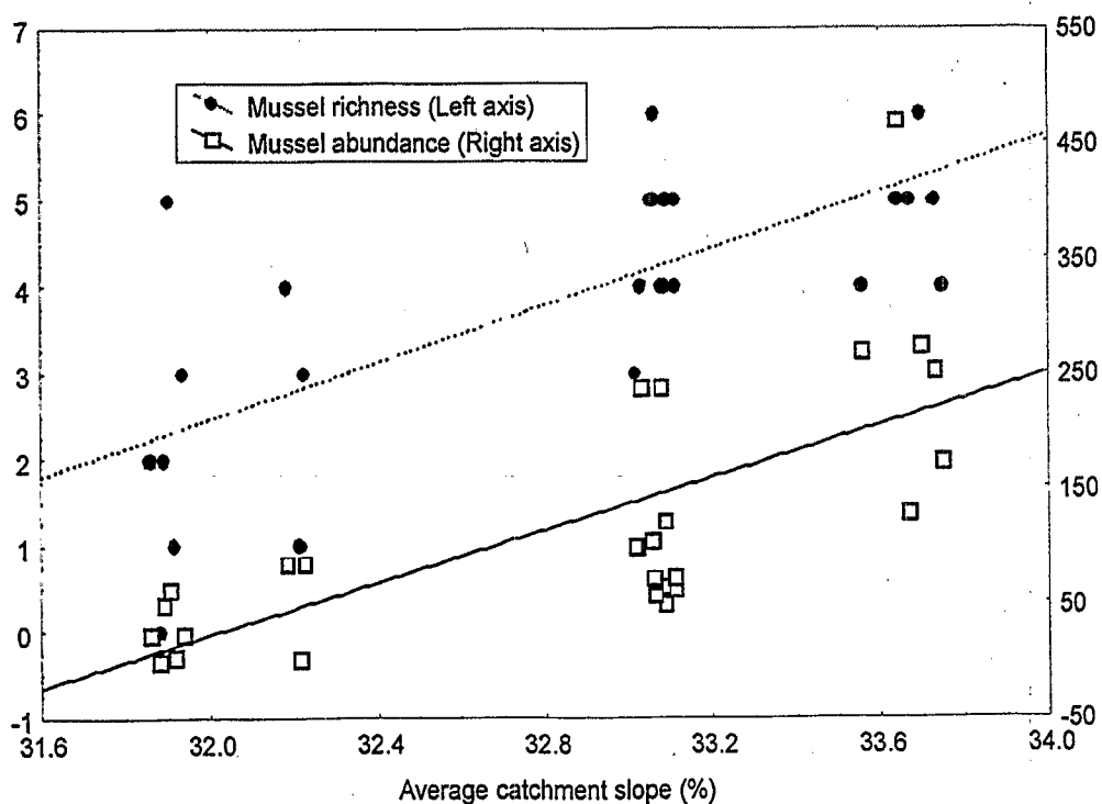
Figure C-8. Relation of mussel richness (left Y-axis) and abundance (right Y-axis) to average catchment slope (%) for high-order streams (>4 th order).
