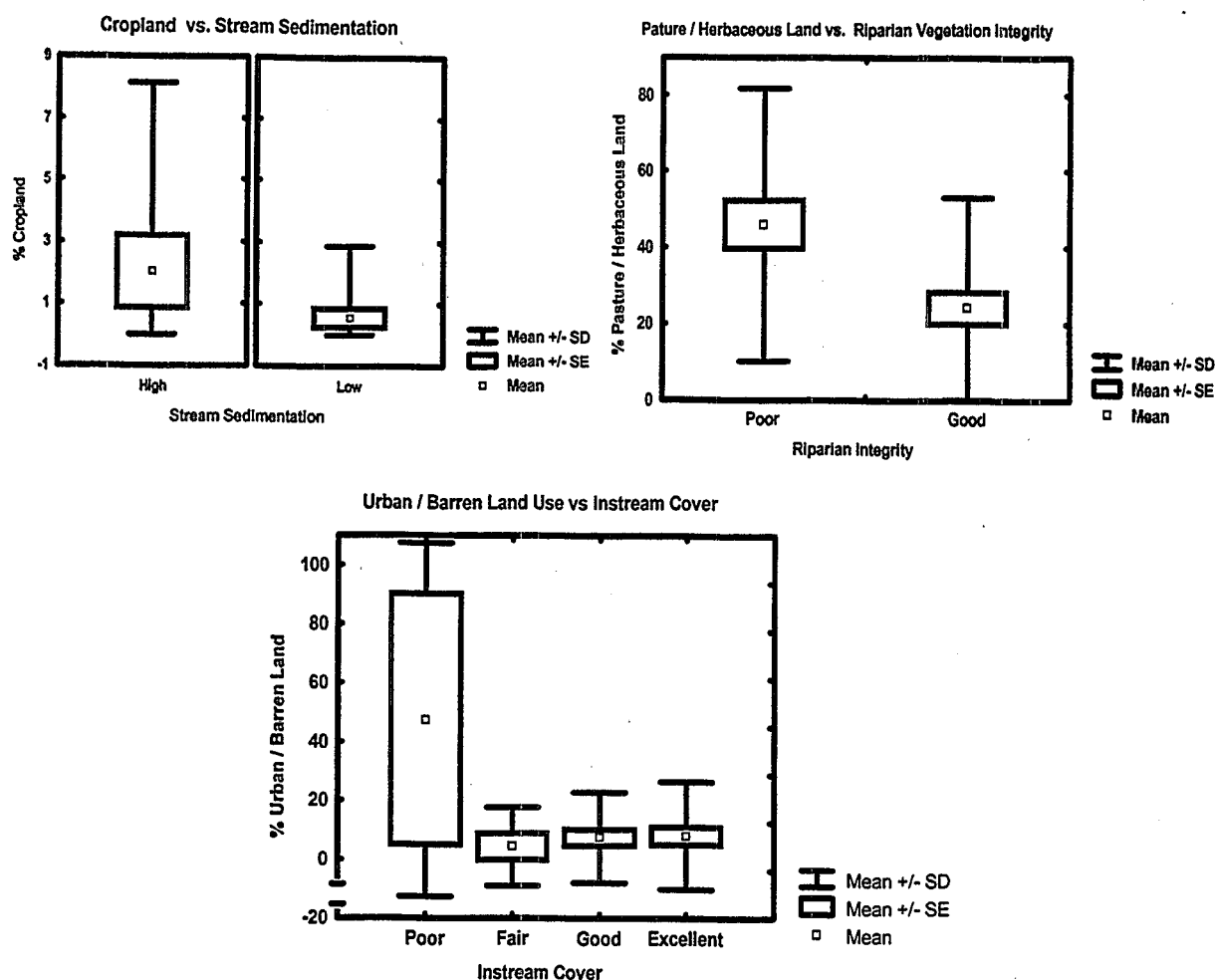
Figure 5-2. Relationships observed between land-use activities and instream habitat measures for sites in the Clinch and Powell watershed, based on TVA's CPRATS dataset and a restricted elevation range of 350–450 m (N = 85).
