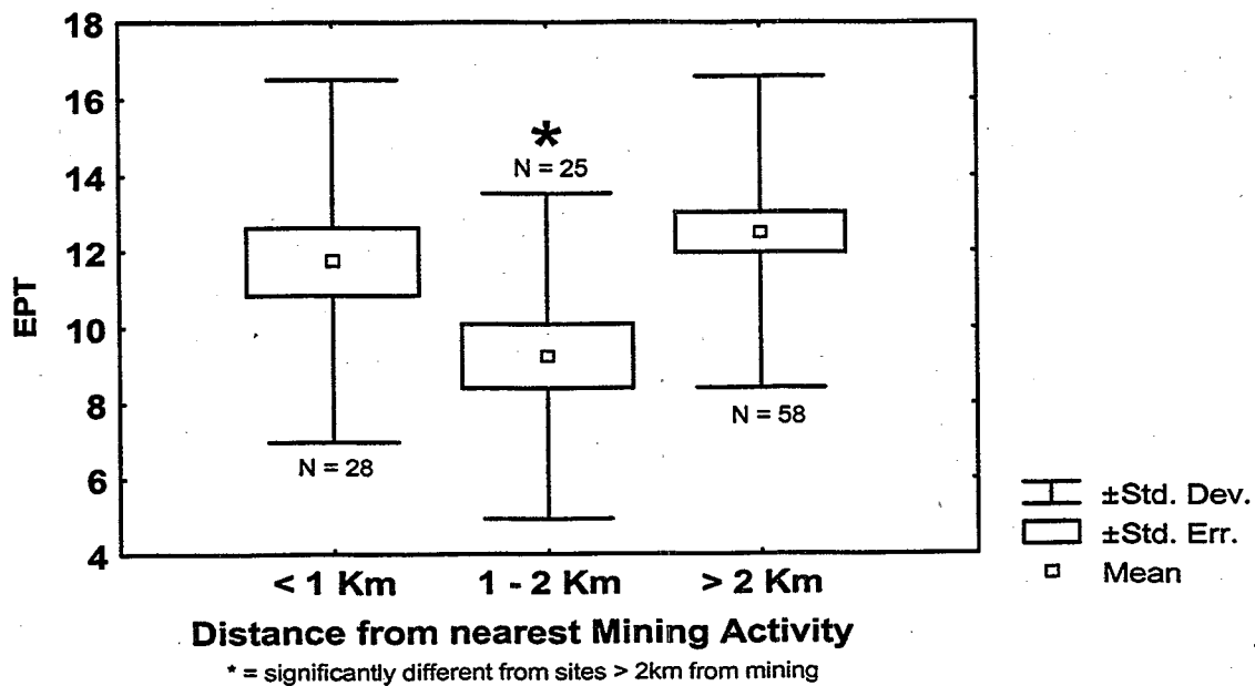
Figure 5-5. Fish IBI or insect EPT values in relation to proximity to coal mining sources. Data derived from TVA's CPRATS dataset (1995–1997).
