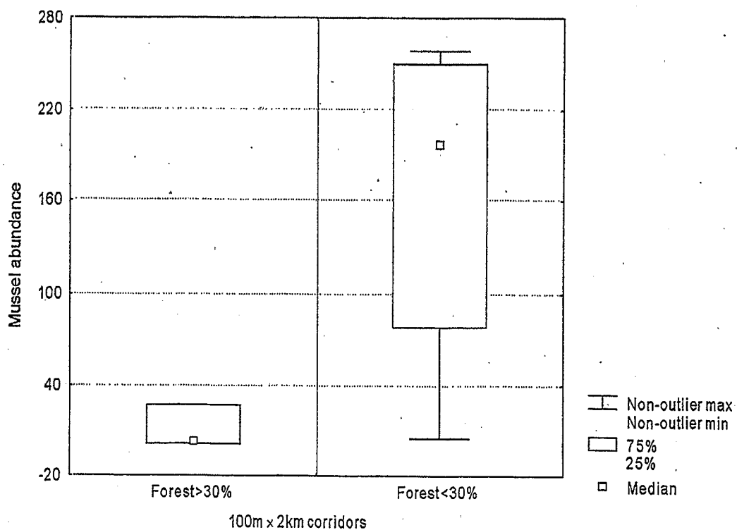
Figure C-6. Abundance of mussels in relation to forested land within 100-m-wide, 2-km-long riparian corridors of low-order streams (>4 th order).
