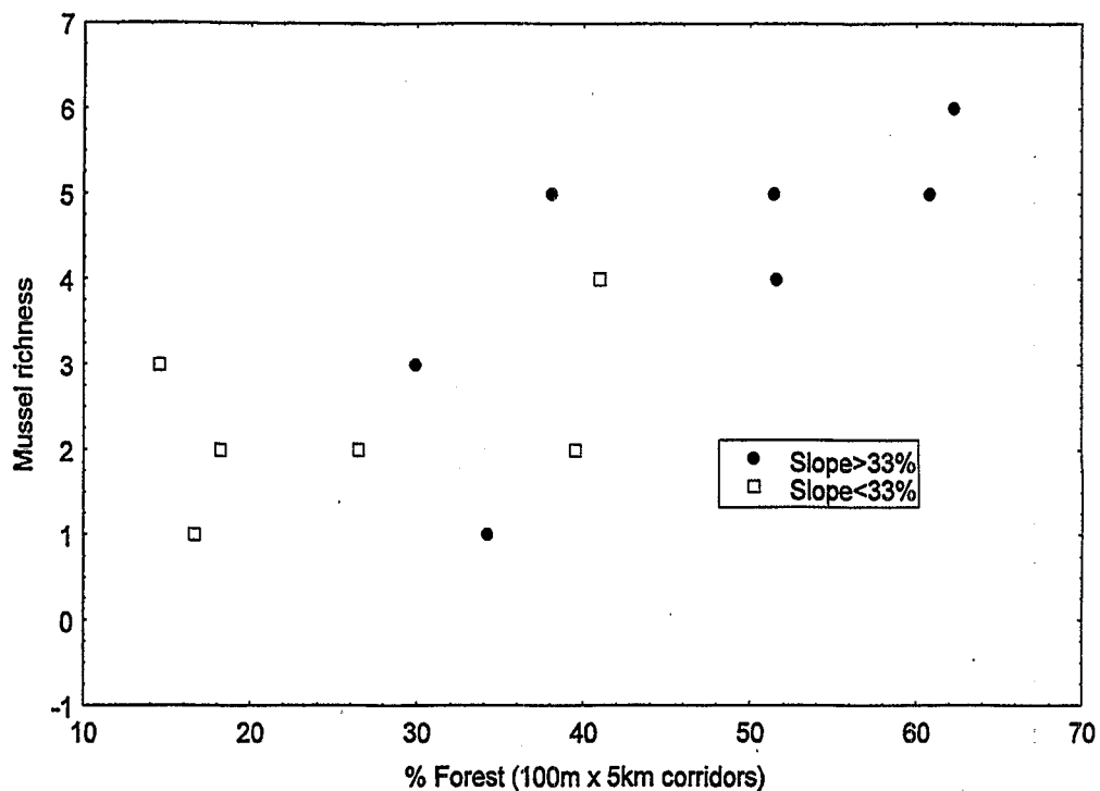
Figure C-1. Mussel richness versus the percentage of forested land within 100-m- wide, 5-km-long riparian corridors; streams are separated according to an average catchment slope threshold of 33%.
