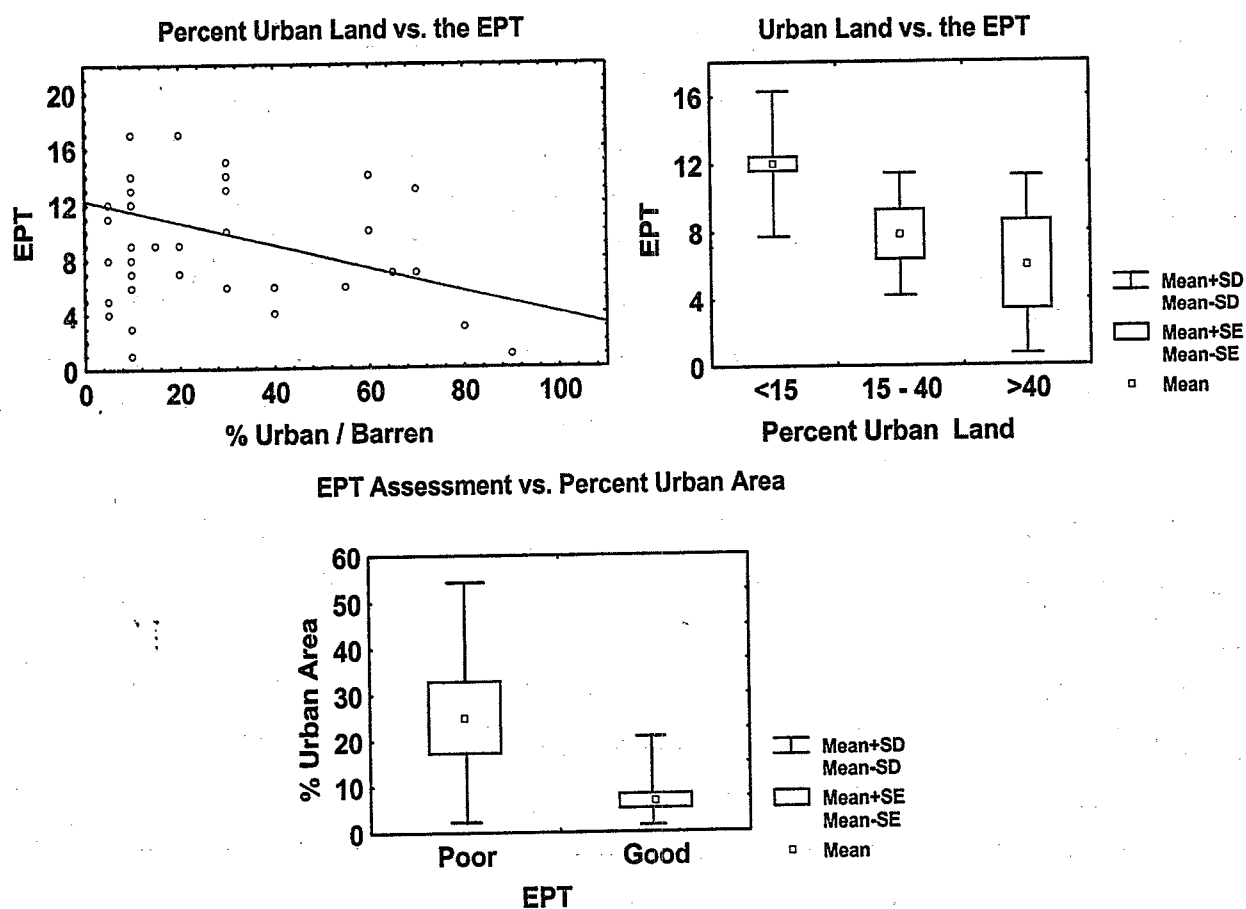
Figure 5-9. Significant relationships between land-use activities or habitat quality and invertebrate EPT score. ( R^2 = 0.29 )
