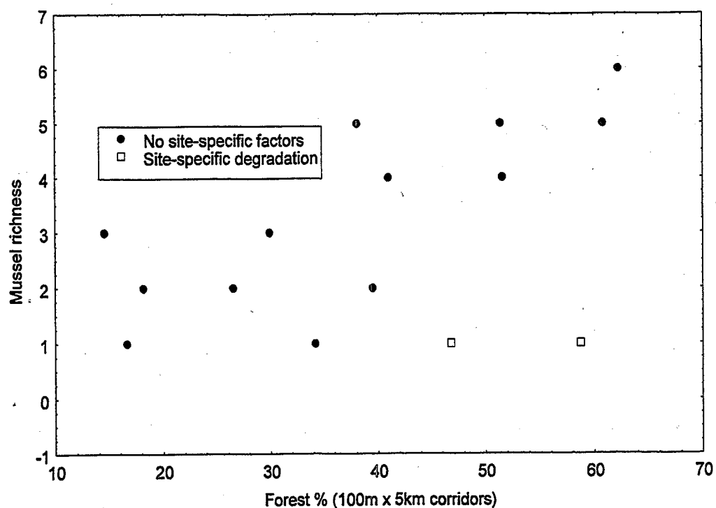
Figure C-13. Mussel richness versus corridor forested land for both sites with specific stressors and those with no site-specific stressors; site-specific degradation is seen here as outlier sites from broad-scale patterns.
