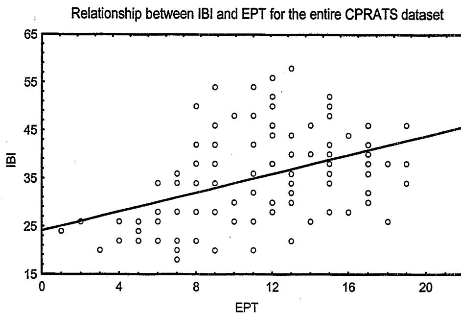
Figure 4-8. Relationships between benthic insect EPT and fish IBI values for TVA CPRATS sites (1995–96) in Copper Creek alone and for the entire Clinch and Powell CPRATS dataset.
