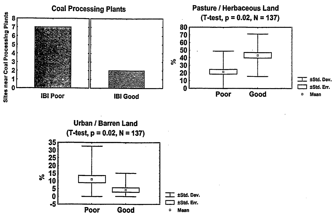
Figure 5-4. Significant relationships observed between land-use sources and the IBI for the entire CPRATS data set ( N = 155 ).
