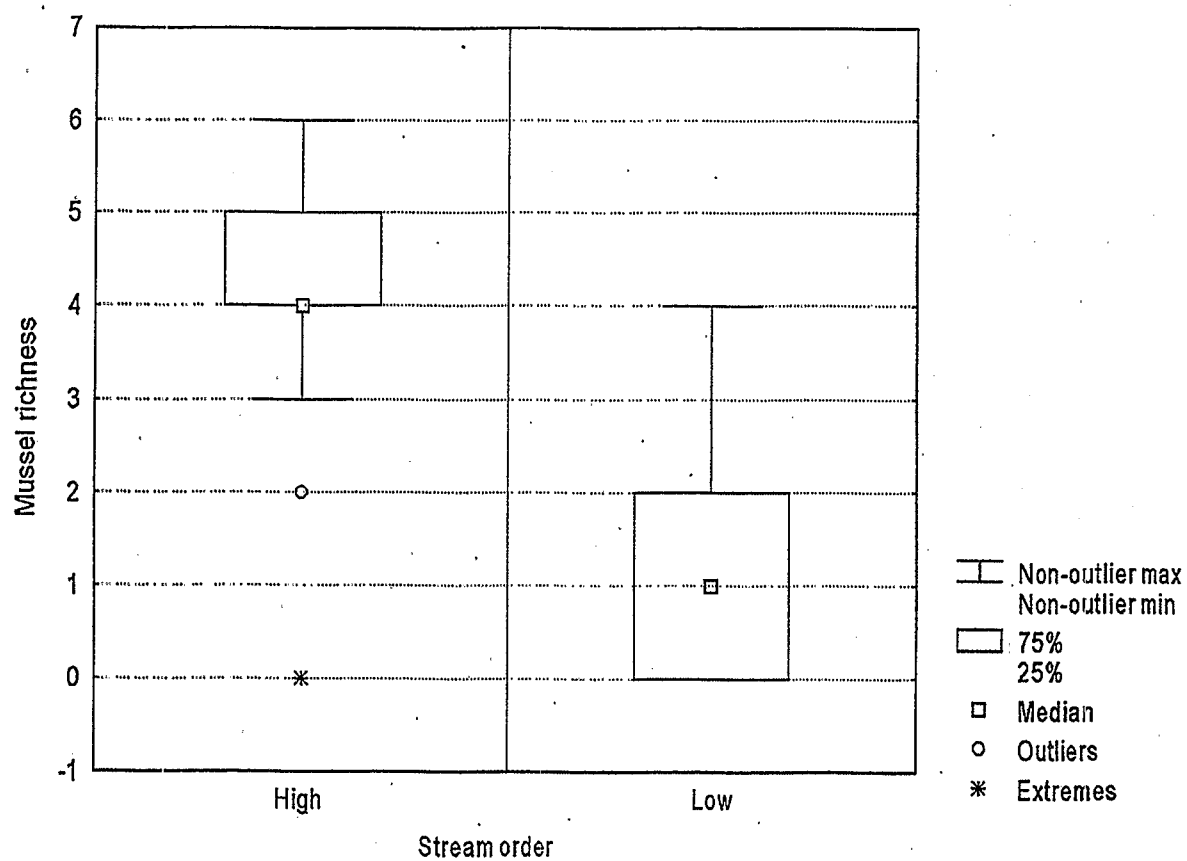
Figure C-4. Mussel richness in high (>4 th order) and low (3-4 th order) order streams.
