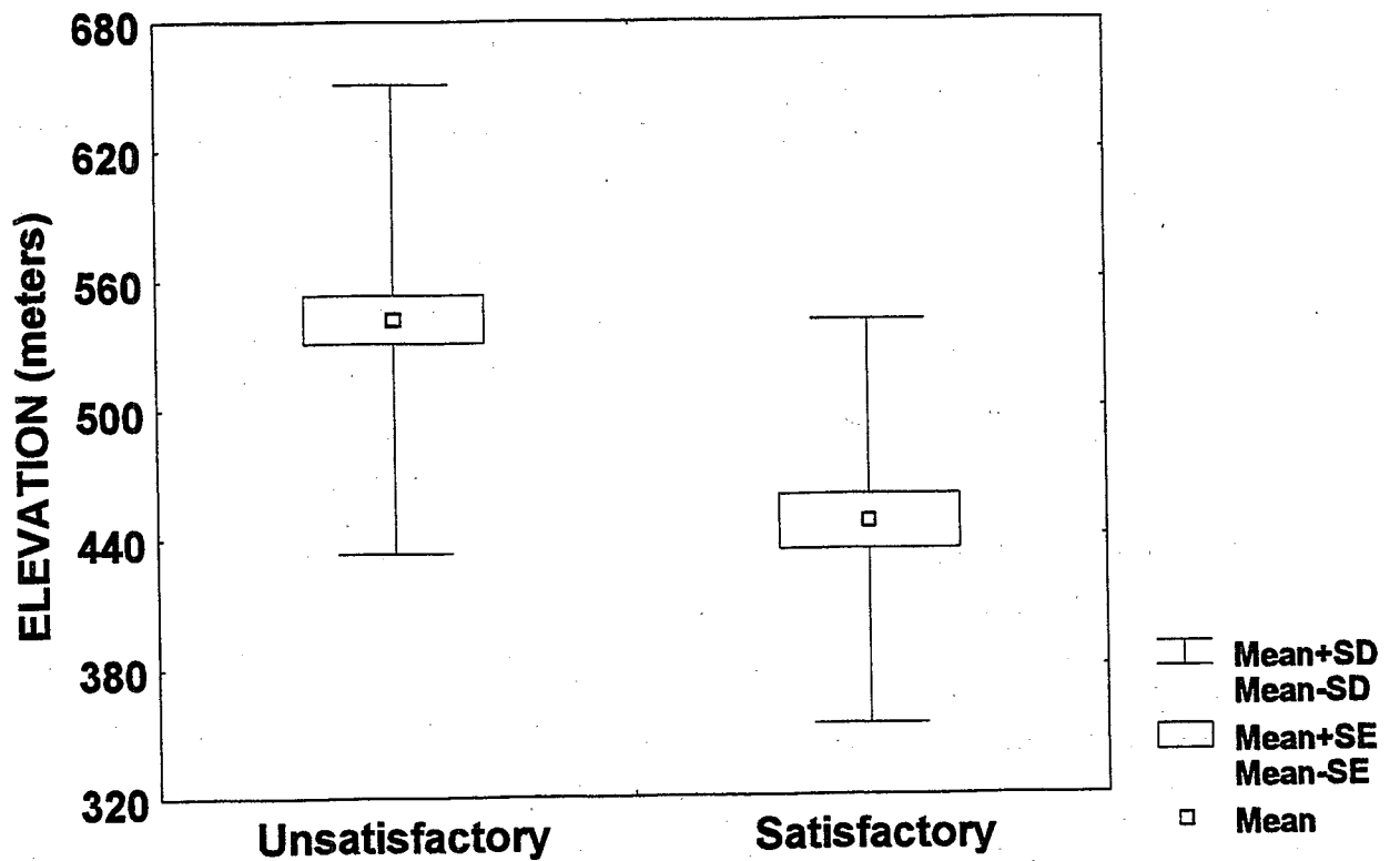
Figure 5-1. Relationship between the fish IBI and stream elevation, with the IBI expressed as either a continuous variable (upper figure) or as a categorical variable (lower figure), based on TVA's ratings.
