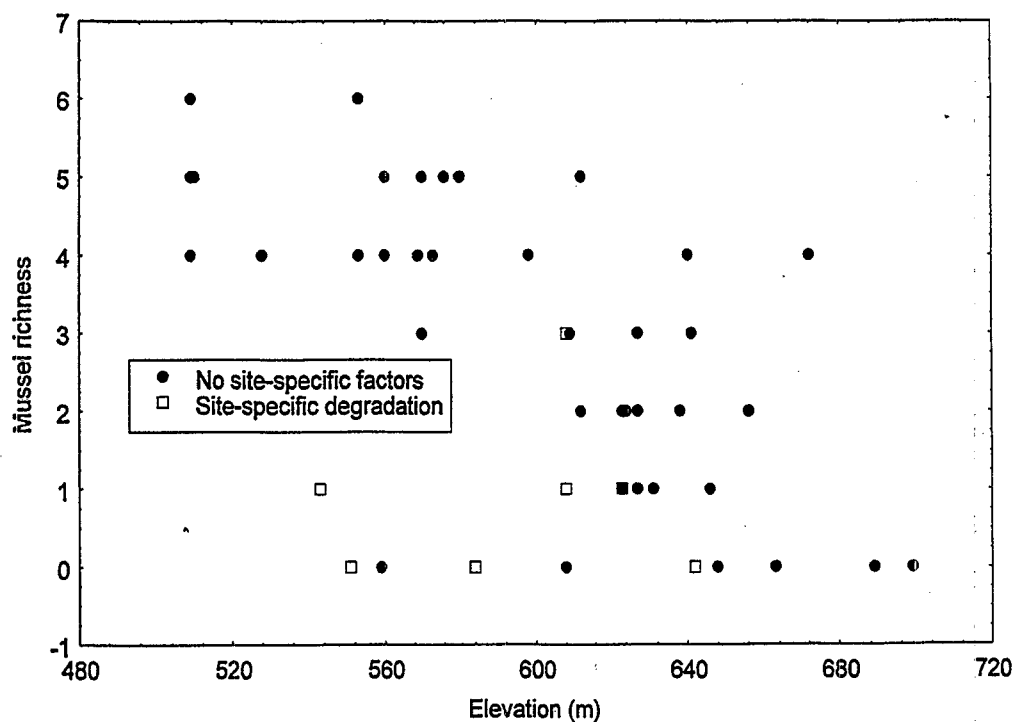
Figure C-12. Mussel richness versus site elevation for both sites with specific stressors and those with no site-specific stressors; site-specific degradation is seen here as outlier sites from broad-scale patterns.
