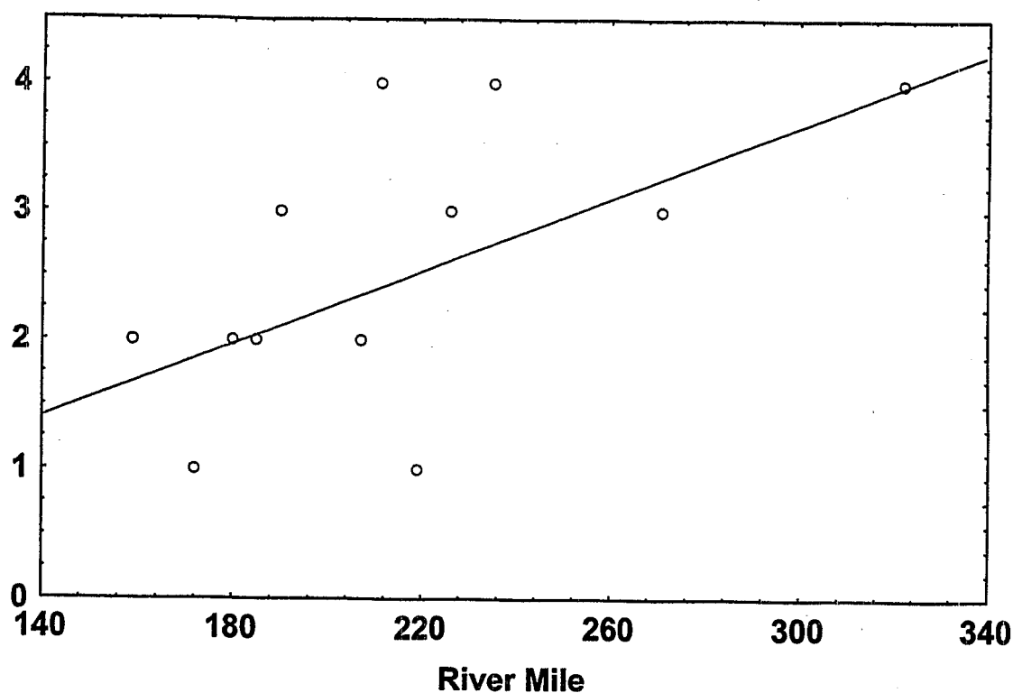
Figure 5-16. Mean number of cumulative sources of stress as one progresses upstream in the Clinch River ( r = 0.74 ).
