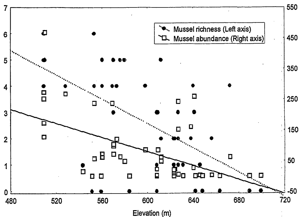
Figure C-7. Relation of mussel richness (left Y-axis) and abundance (right Y-axis) to site elevation (m) for high-order streams (>4 th order).
