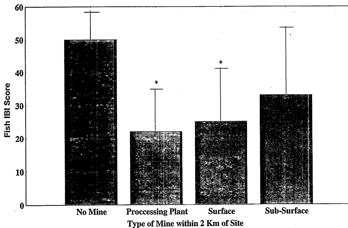
Figure 5-7. Effect of mine type on fish community integrity as a function of the type of mine.
