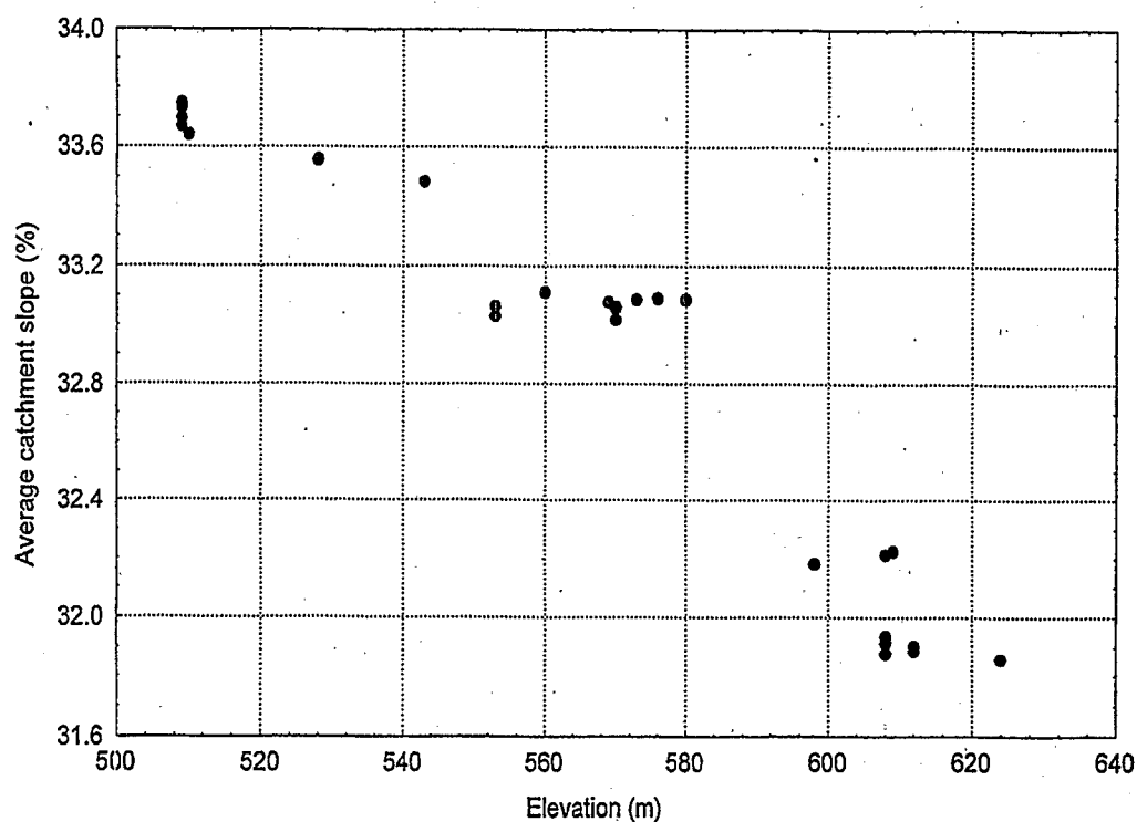
Figure C-9. Site elevation (m) versus average catchment slope (%) for high-order streams (>4 th order).
