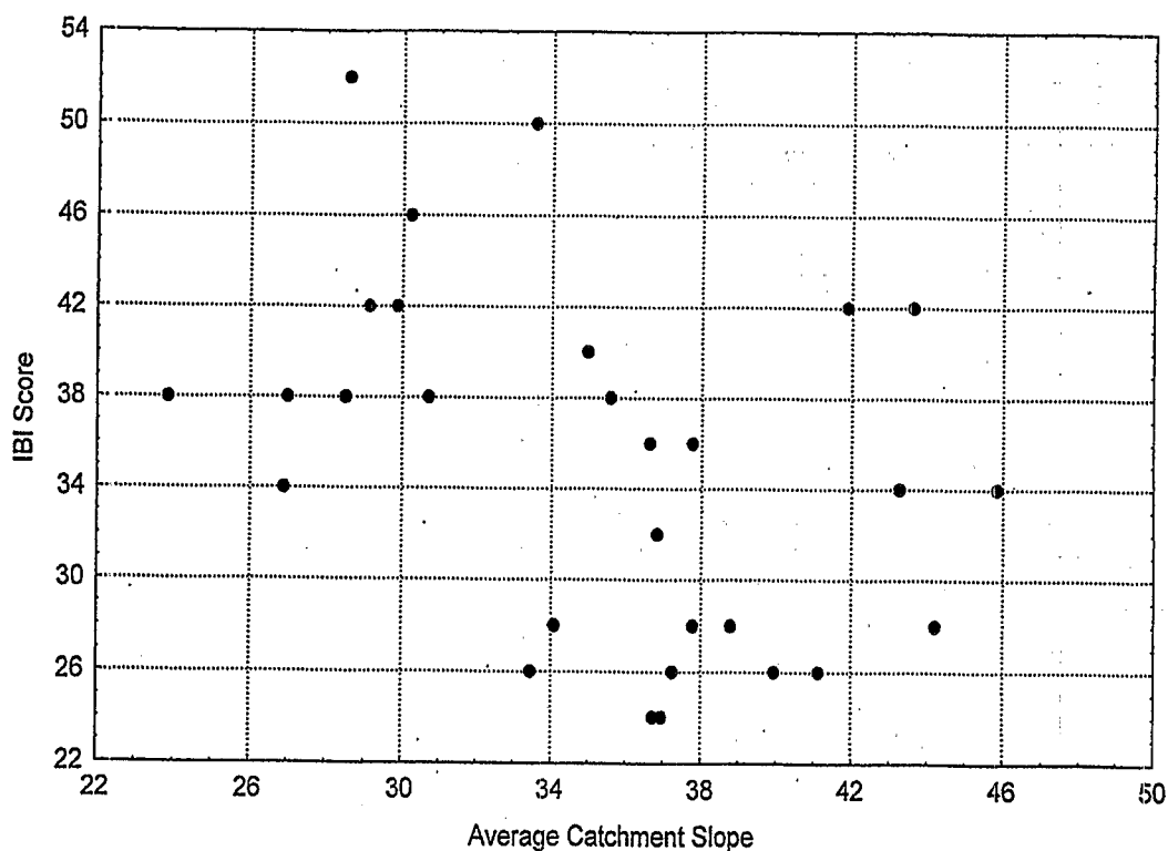
Figure 5-20. IBI score versus average catchment slope (%).
