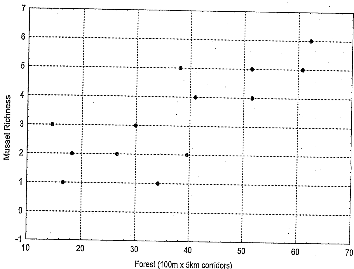
Figure 5-19. Mussel richness versus percent forested land use in 100-m-wide, 5-km-long riparian corridors.
