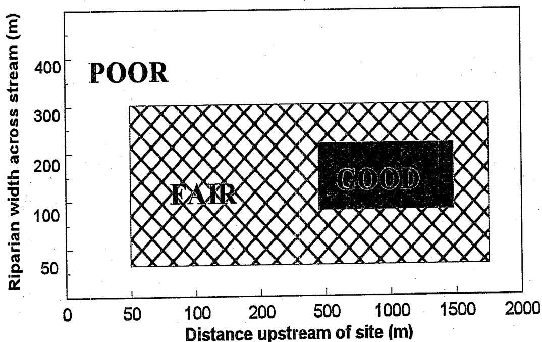
Figure 4-3. Illustration depicting the strength of relationships between land uses and biological measures as a function of riparian buffer width and distance upstream.
