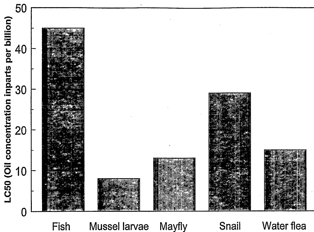
Figure 5-6. Comparison of acute toxicity results ( LC_{50} ) for several species, based on laboratory water exposures of a hydraulic oil commonly used in coal longwall mining machinery in the Powell River subwatershed. The higher the LC_{50} , the less toxic the chemical. Actual species tested included Pimephales promelas (fathead minnow), Villosa spp. (mussel), Stenonema spp. (mayfly), Physella spp. (snail), and Ceriodaphnia dubia (water flea).
